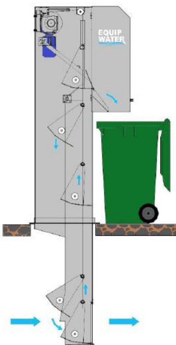
Vertical Bar Screen Operation
